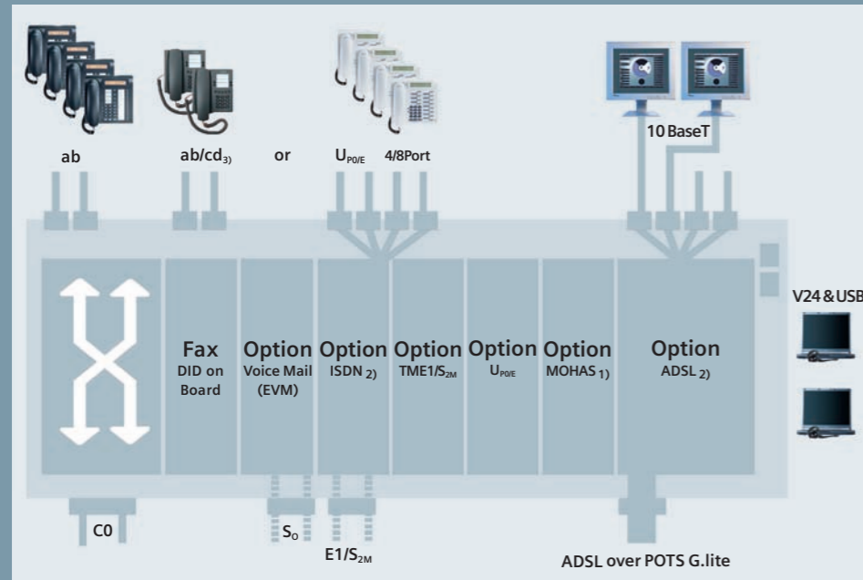
HiPath 1100 V6.0/7.0 technical data
